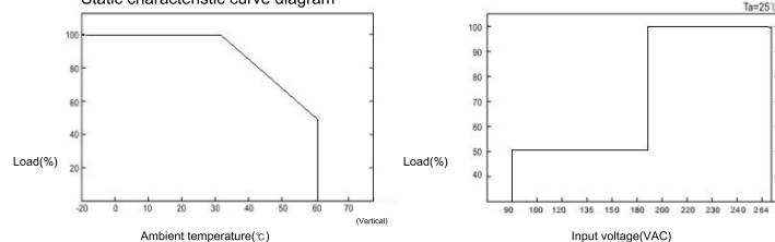
Static characteristic curve diagram
